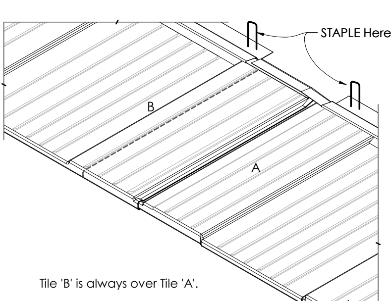
Figure 7.3 Overlap Detail
