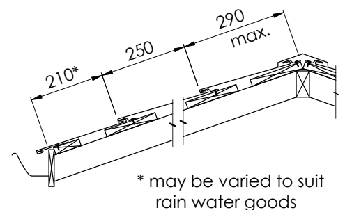
Figure 7.5 Batten Layout
