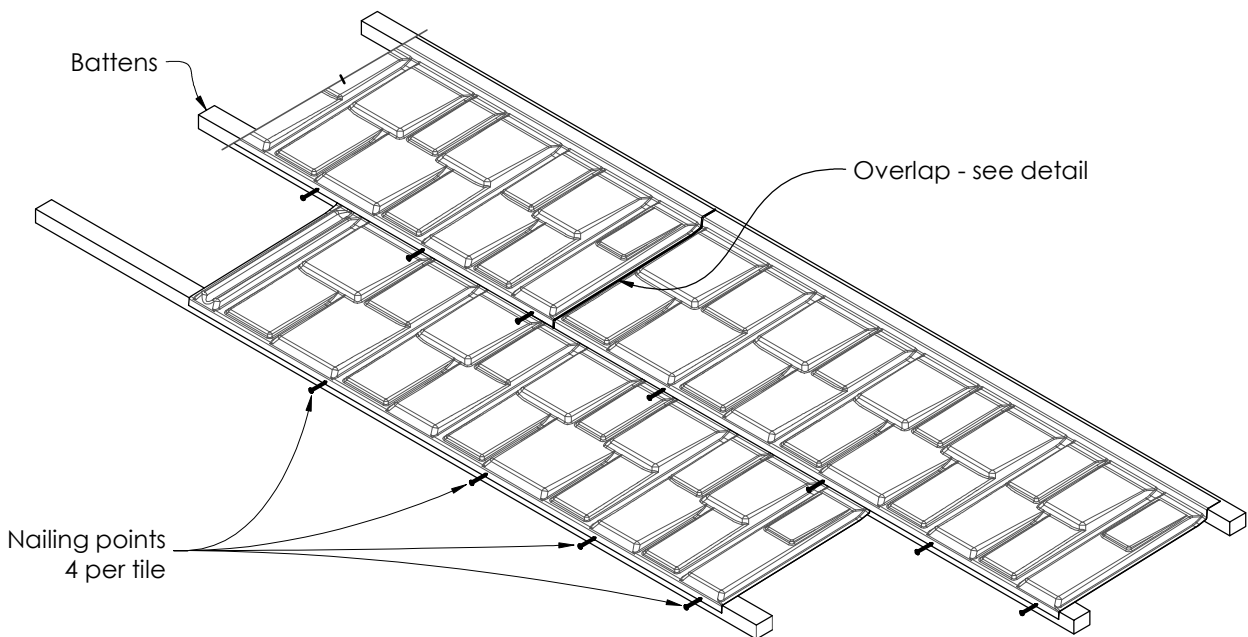
Figure 5.2 Nailing Detail
