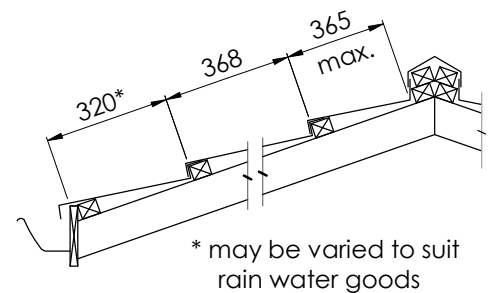
Figure 5.5 Batten Layout
