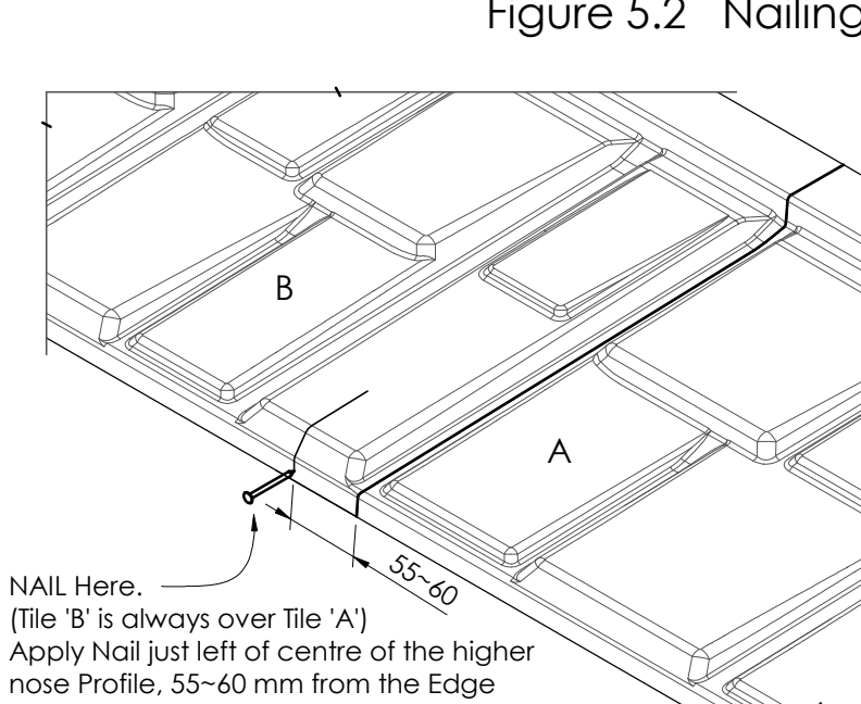
Figure 5.3 Overlap Detail
