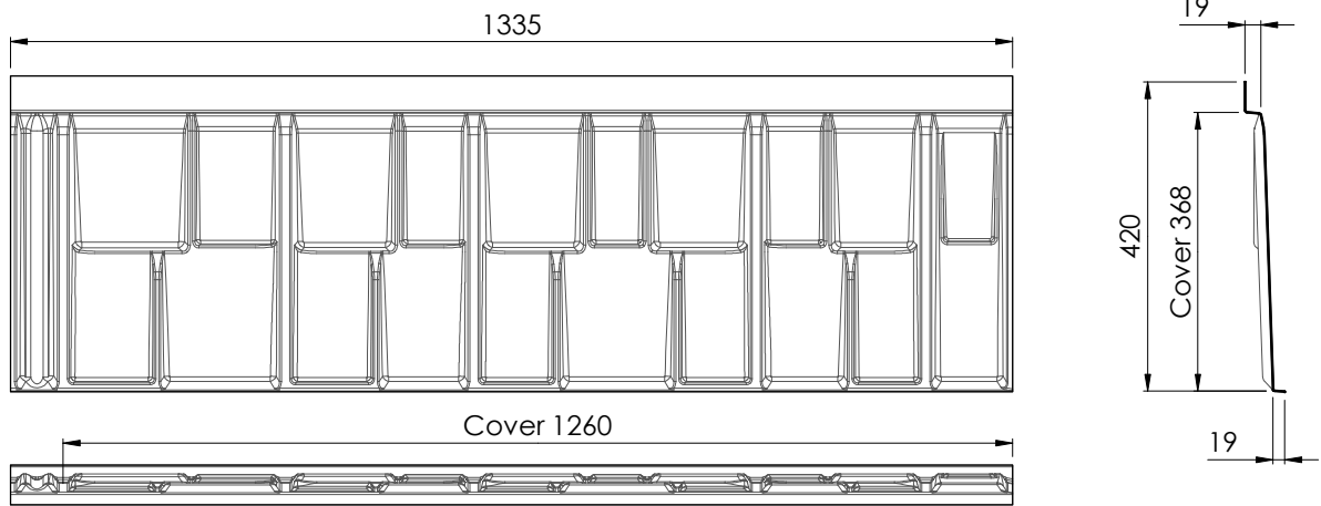
Figure 5.1 Tile Dimensions
