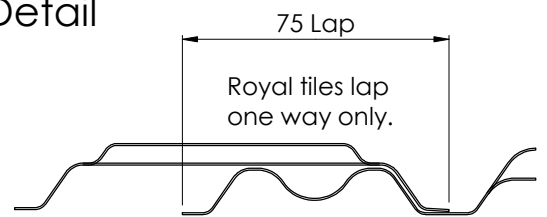
Figure 5.4 Lap Section
